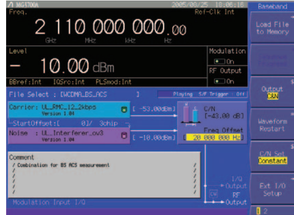
Wanted Signal + Interfering Screen
