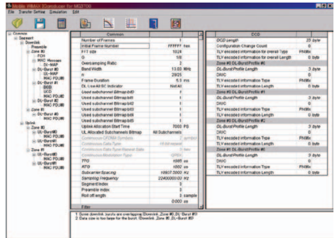
Mobile WiMAX IQproducer Setting Screen
