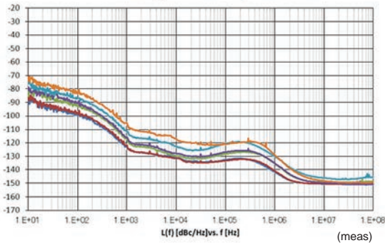
Single sideband phase noise
