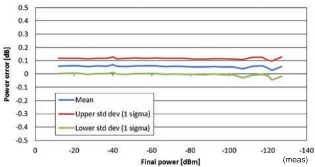
Linearity
